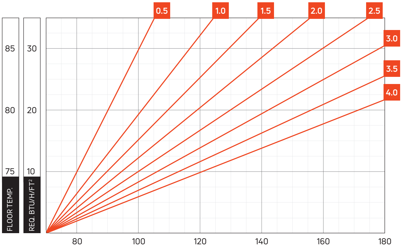
Average of Supply/Return Water Temperature at Manifold for Good Dynamic Performance
