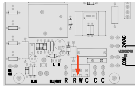
EB-S and EB-MS boards with related wiring label.
