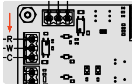
EMB-R1 board with related wiring label.
