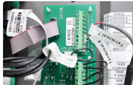
Lochinvar TT screw terminals (7, 8).
