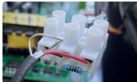
Prefabricated connector with resistor.
