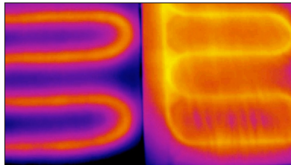
After 2.5 hours, gypsum concrete is producing 10 BTUs/sf, while Warmboard is producing 18 BTUs/sf, with more even surface temperatures. The variation in temperature across the surface of Warmboard is only 2+°F while gypsum concrete has 6°F of variation.
